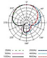
Polar Patterns
